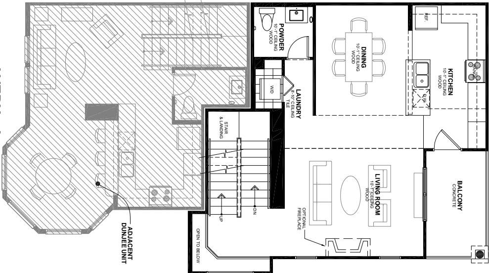
AVERY - A SECOND FLOOR PLAN Scale: 3/32" = 1'-0"
