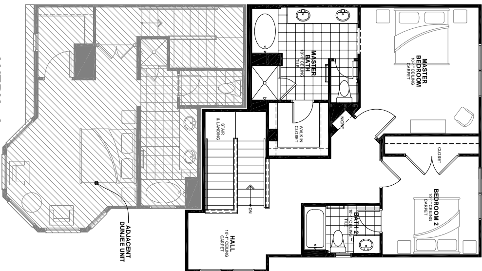
AVERY - A THIRD FLOOR PLAN Scale: 3/32" = 1'-0"
